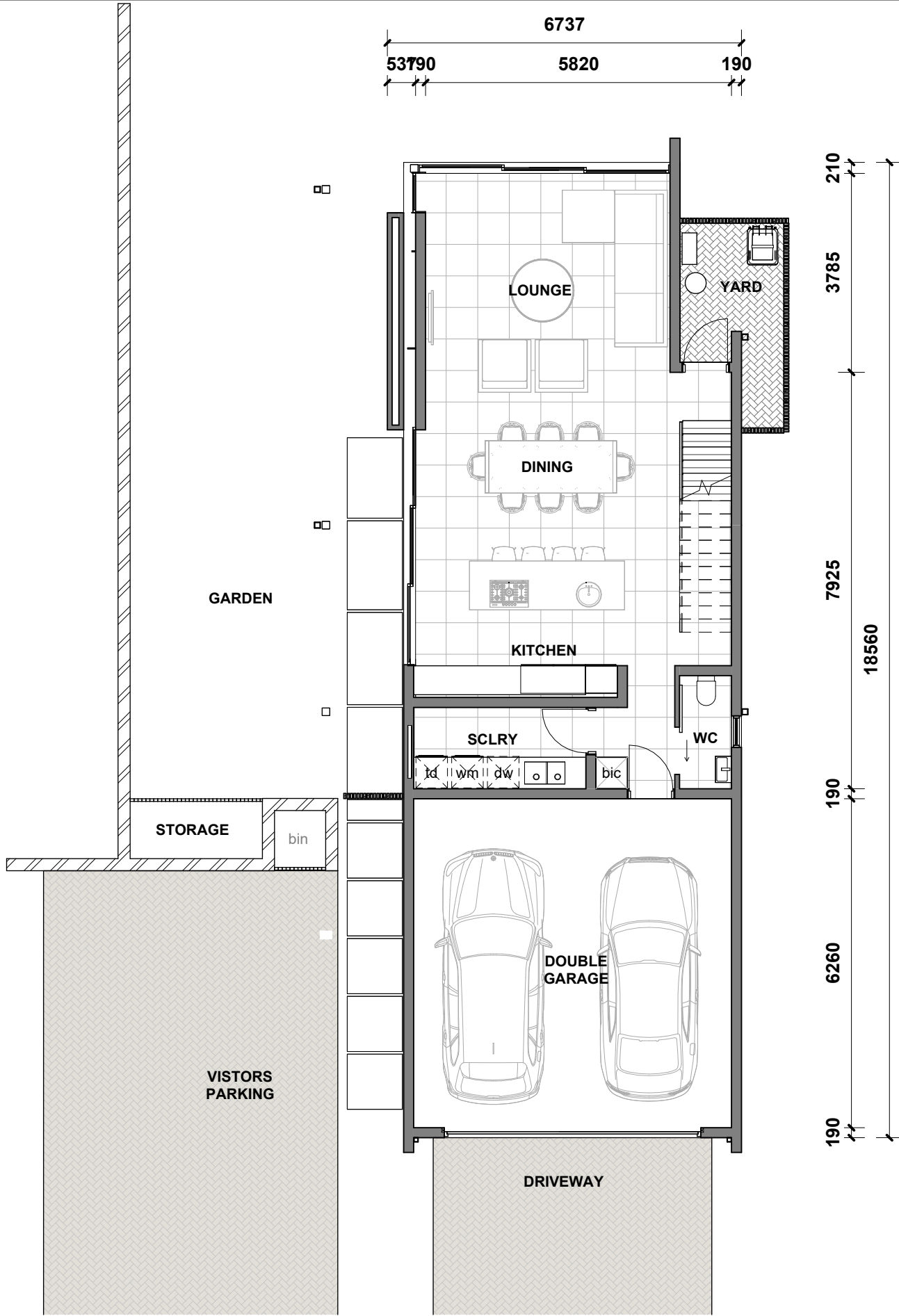
00 - GROUND FLOOR SCALE 1 : 100
